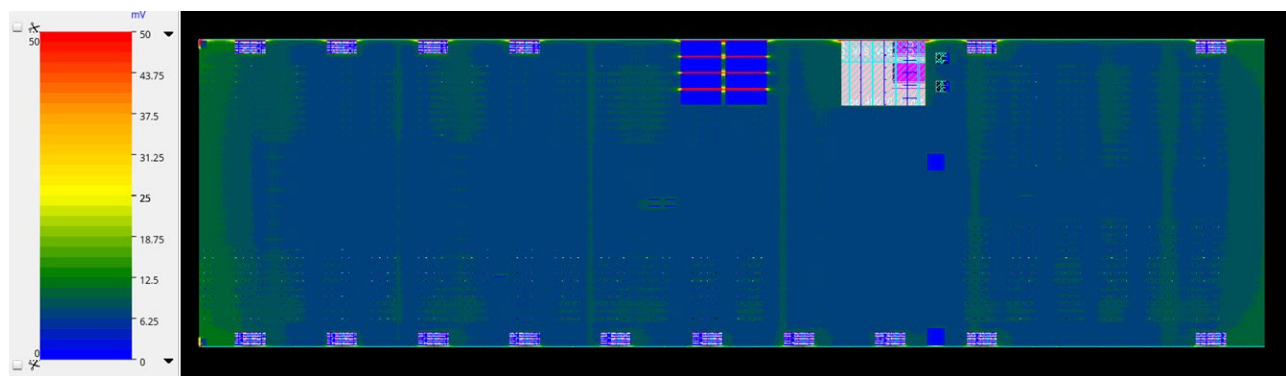
Figure 5-13. Top Die Early Static IR Drop Analysis Results
